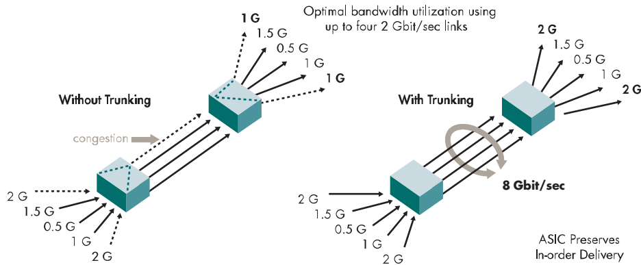
Figure 1. Optional ISL Trunking groups multiple ISLs to enable high-speed data traffic
